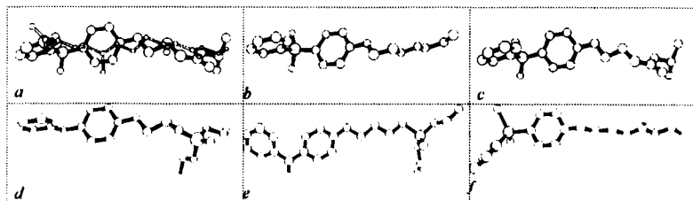
FIGURE 1 Molecular modeling of JH mimetics: a - the superimposed model of JH-III and compound 2a ; b - compound 2b ; c - compound 2a ; d - compound 1a ; e - compound 1b ; f - compound 3a
